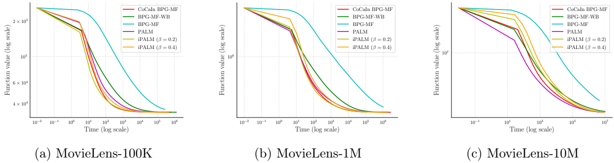
Figure 7: Time plots for Matrix Completion on MovieLens Datasets [29].
