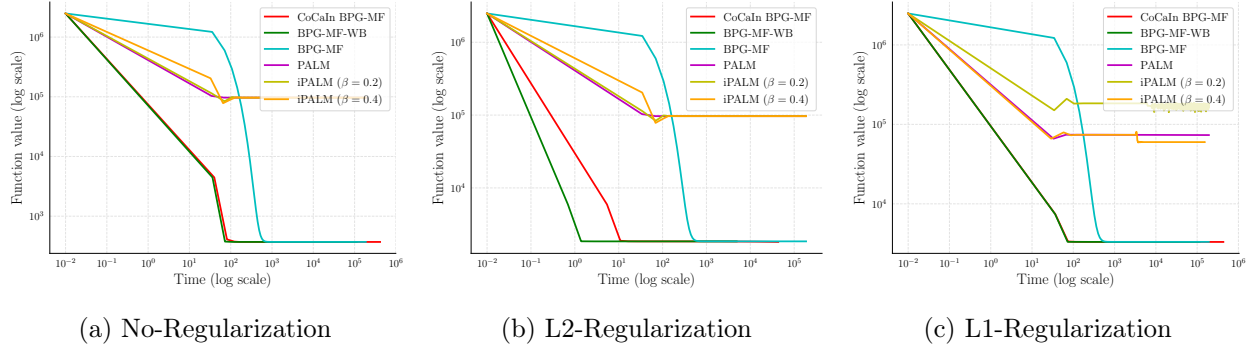
Figure 6: Time plots for Non-negative Matrix Factorization on Medulloblastoma dataset [11].
